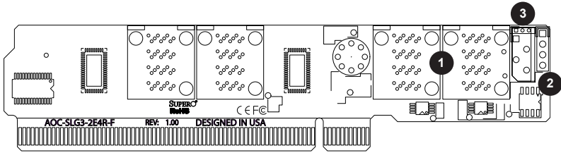
Figure 2-2. AOC-SLG3-2E4R-F Layout
