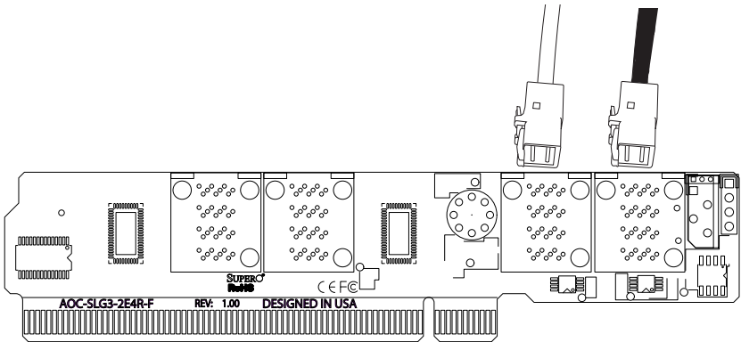
Figure 3-2. Connecting the Cables
