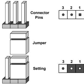
Figure 2-4. Front Jumpers
