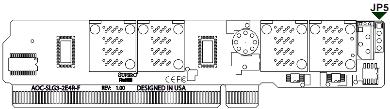
Figure 2-4. Front Jumpers
