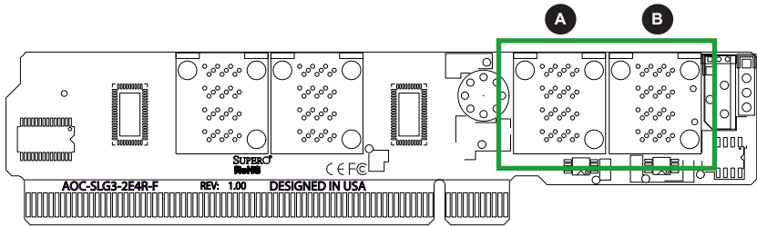
Figure 2-3. NVMe Connectors
