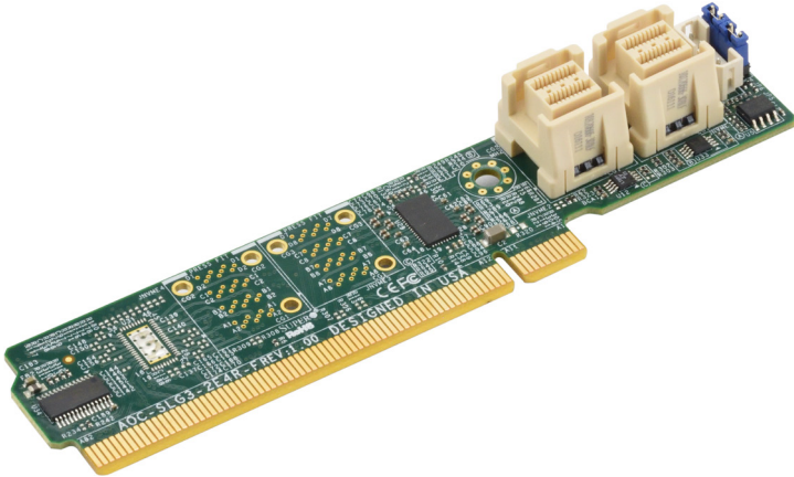
Figure 2-1. AOC-SLG3-2E4R-F
