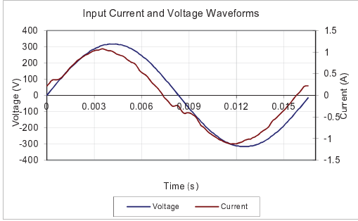
Input AC Current Waveform (ITHD = 8.76%, 50% Load)
